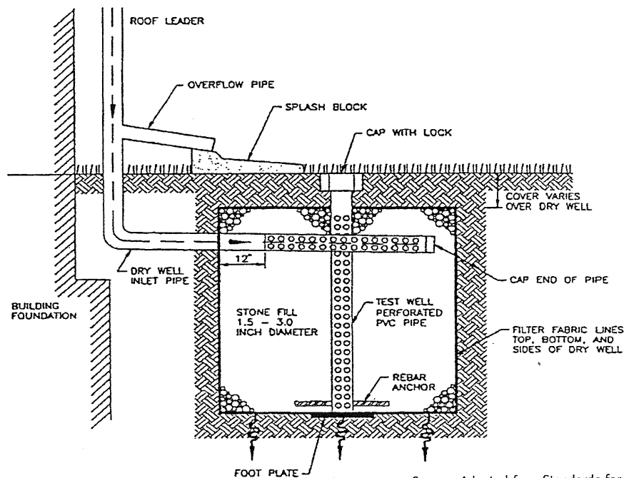
Figure 9.3-1: Dry Well Components
